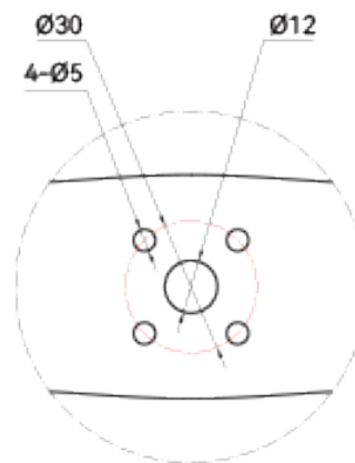
Partial View Scale 2:1
